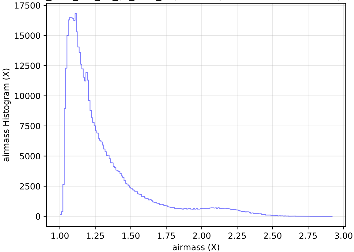
too_elab_r64_d2_gz_v3.4_10yrs All sky r band: airmass Histogram
