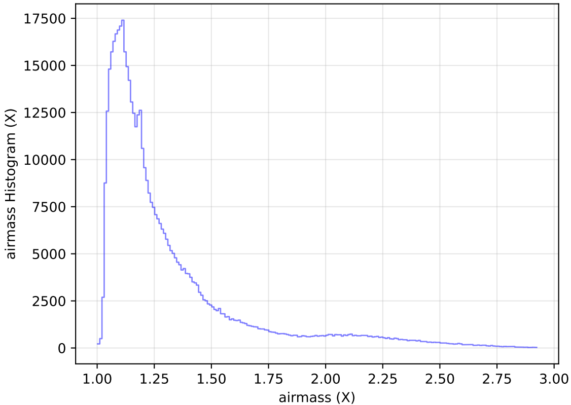
too_elab_r64_d2_gz_v3.4_10yrs All sky i band: airmass Histogram
