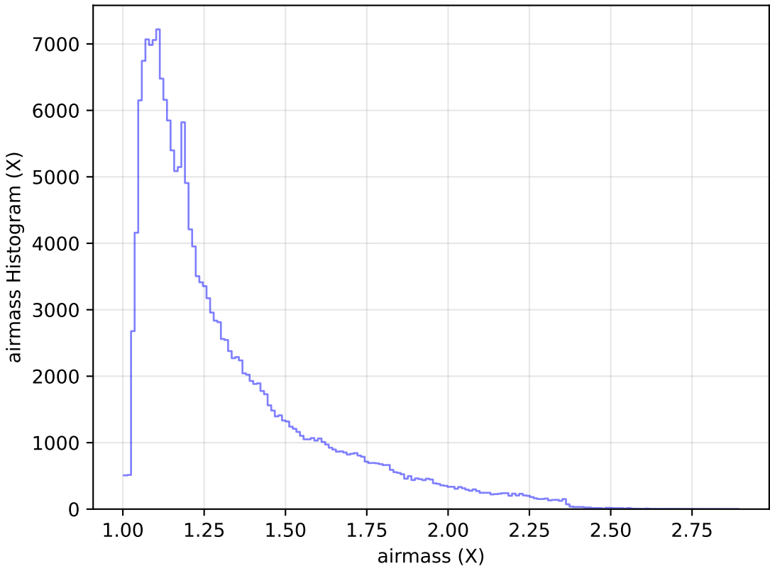
too_elab_r64_d2_gz_v3.4_10yrs All sky g band: airmass Histogram
