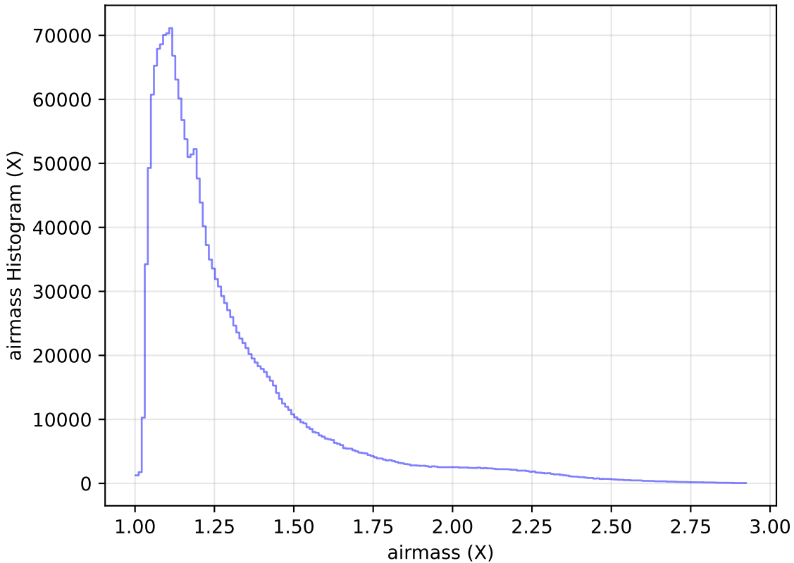
too_elab_r64_d2_gz_v3.4_10yrs All sky all bands: airmass Histogram
