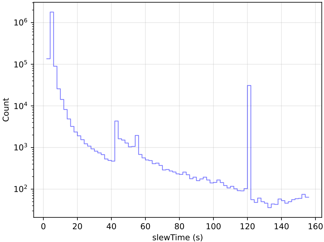
too_elab_r64_d2_gz_v3.4_10yrs All visits: Slew Time Histogram
