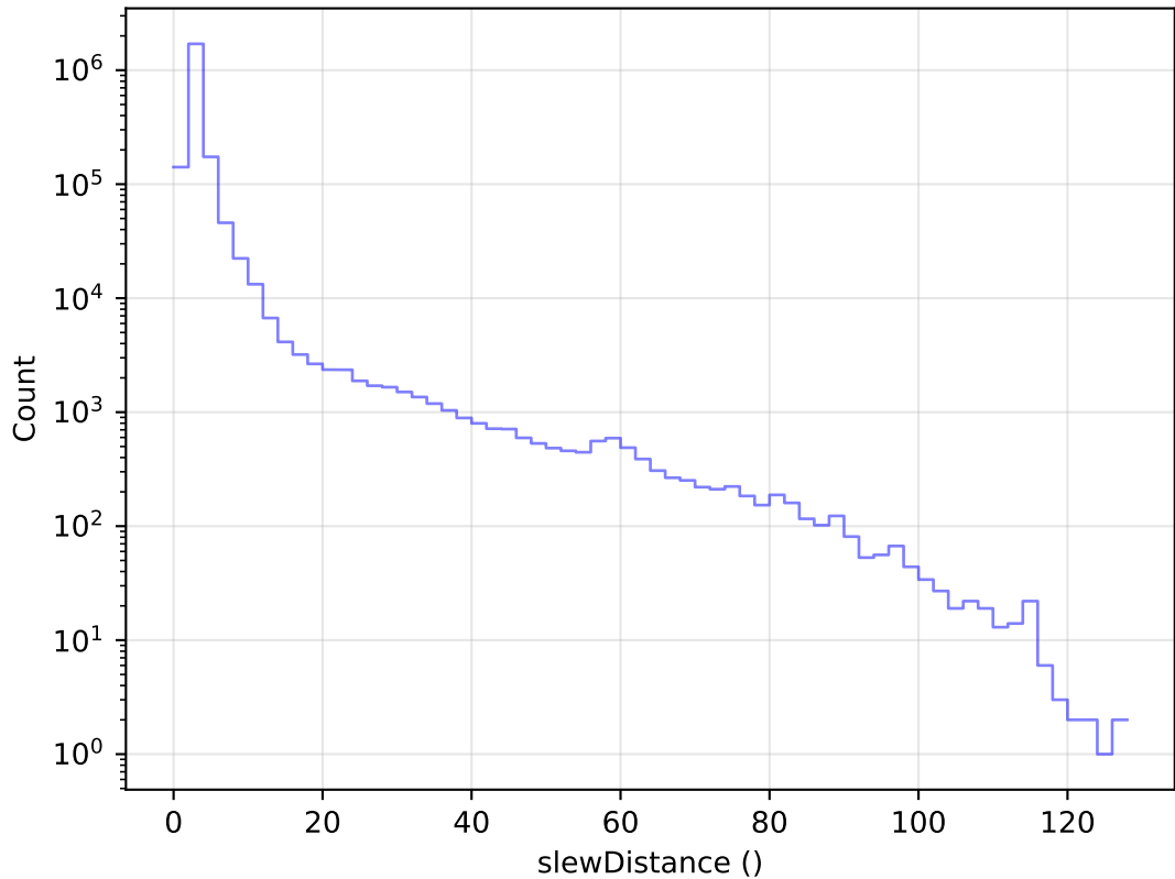
too_elab_r64_d2_gz_v3.4_10yrs All visits: Slew Distance Histogram
