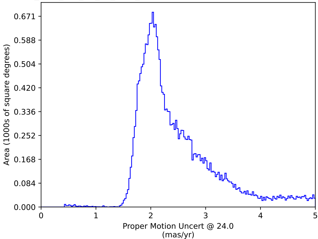
too_elab_r64_d2_gz_v3.4_10yrs All sky: Proper Motion Uncert @ 24.0
