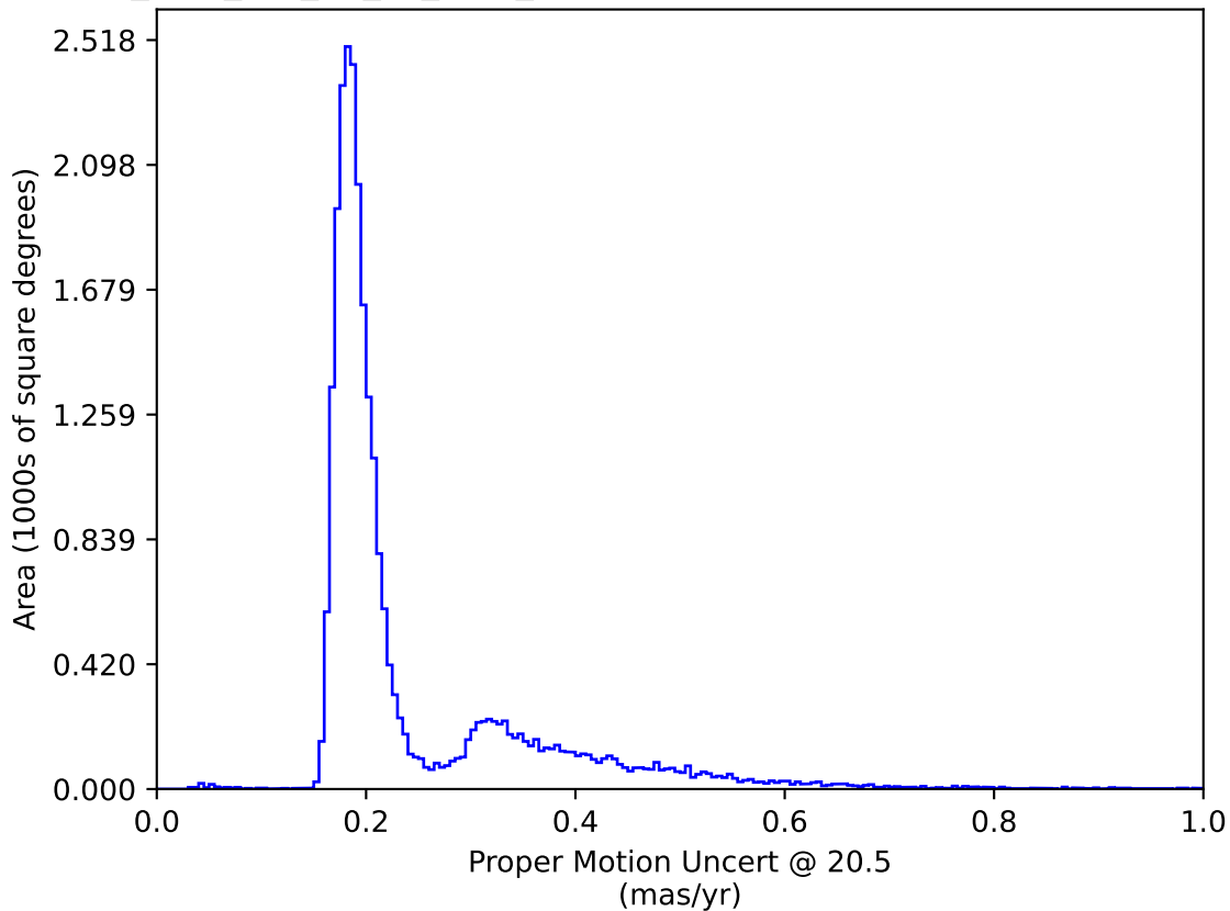
too_elab_r64_d2_gz_v3.4_10yrs All sky: Proper Motion Uncert @ 20.5
