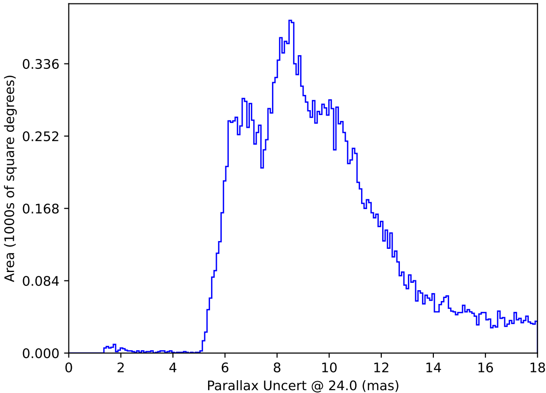
too_elab_r64_d2_gz_v3.4_10yrs All sky: Parallax Uncert @ 24.0
