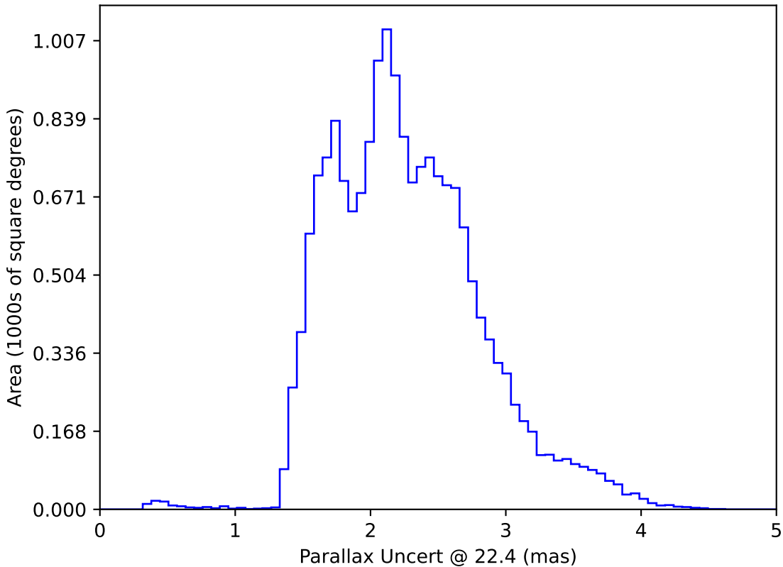
too_elab_r64_d2_gz_v3.4_10yrs WFD: Parallax Uncert @ 22.4
