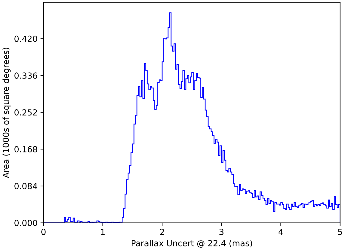
too_elab_r64_d2_gz_v3.4_10yrs All sky: Parallax Uncert @ 22.4
