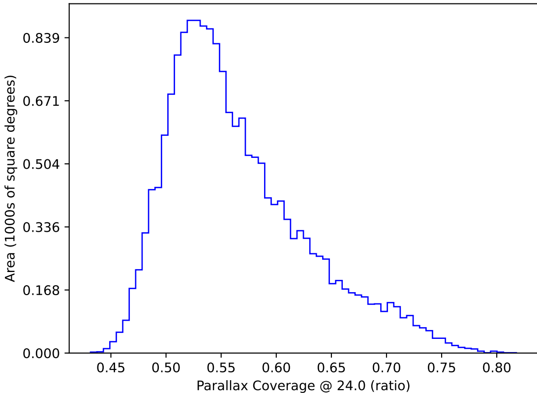
too_elab_r64_d2_gz_v3.4_10yrs WFD: Parallax Coverage @ 24.0
