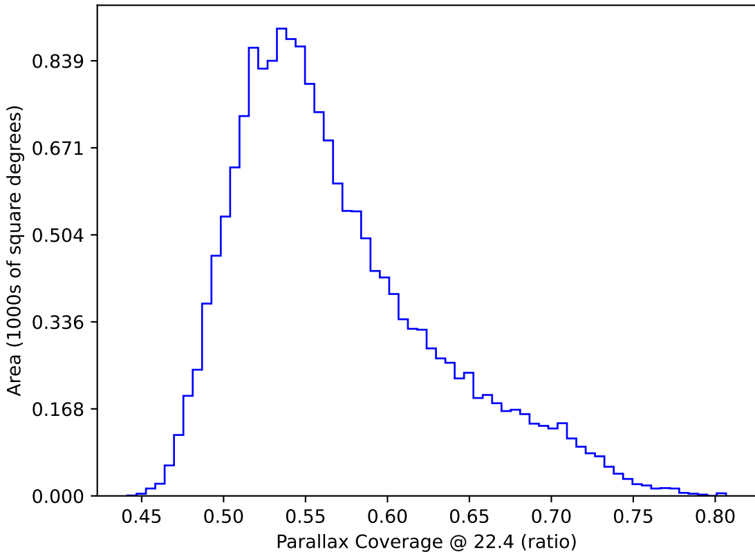
too_elab_r64_d2_gz_v3.4_10yrs WFD: Parallax Coverage @ 22.4
