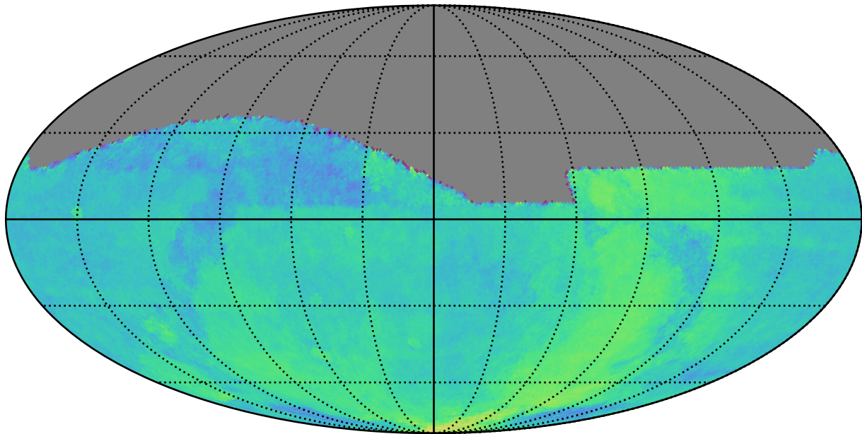
too_elab_r64_d2_gz_v3.4_10yrs All sky: Parallax Coverage @ 22.4
