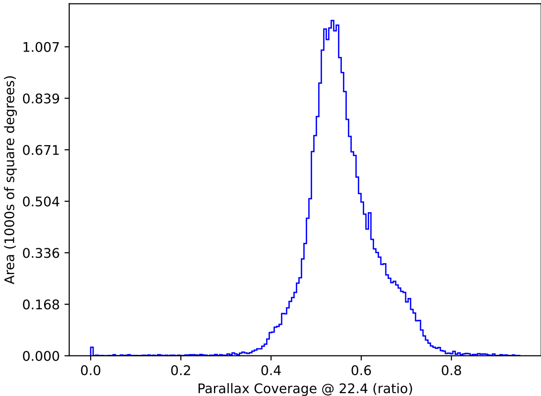
too_elab_r64_d2_gz_v3.4_10yrs All sky: Parallax Coverage @ 22.4
