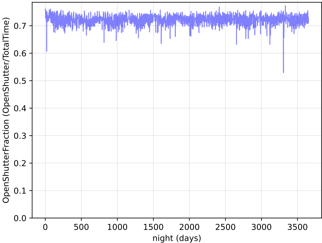
too_elab_r64_d2_gz_v3.4_10yrs Per night: OpenShutterFraction
