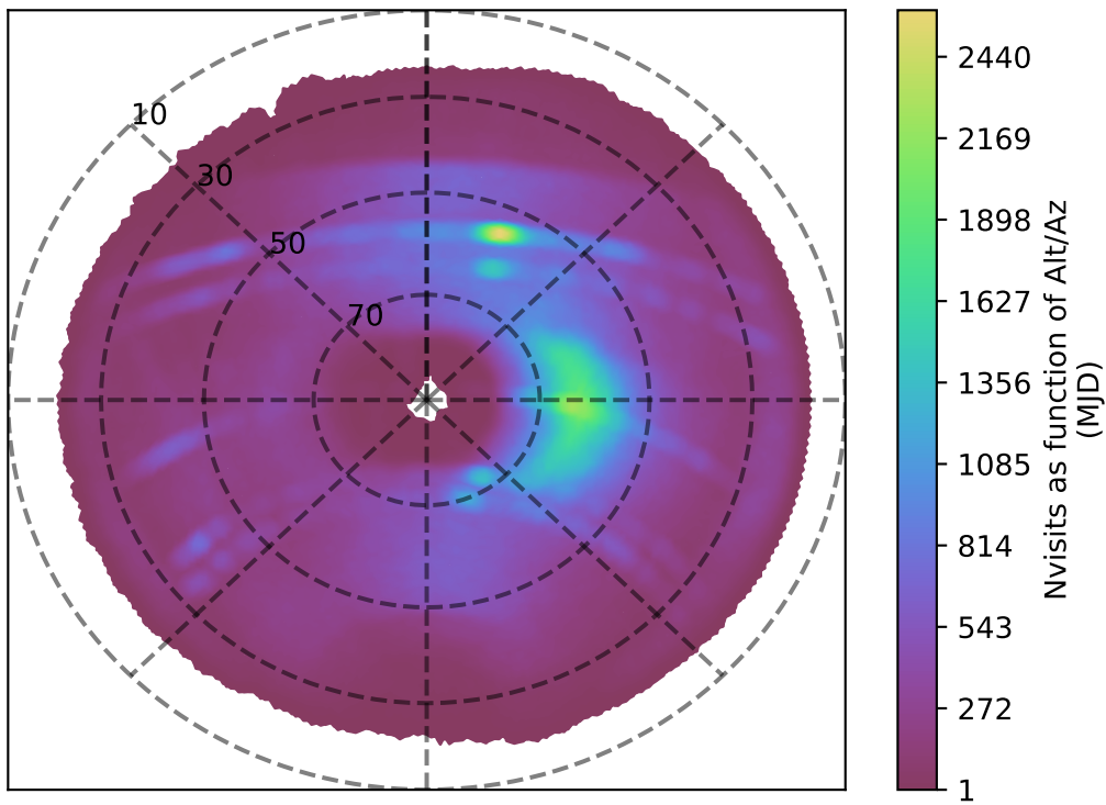
too_elab_r64_d2_gz_v3.4_10yrs z band: Nvisits as function of Alt/Az
