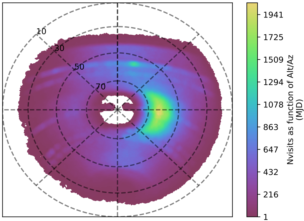
too_elab_r64_d2_gz_v3.4_10yrs y band: Nvisits as function of Alt/Az
