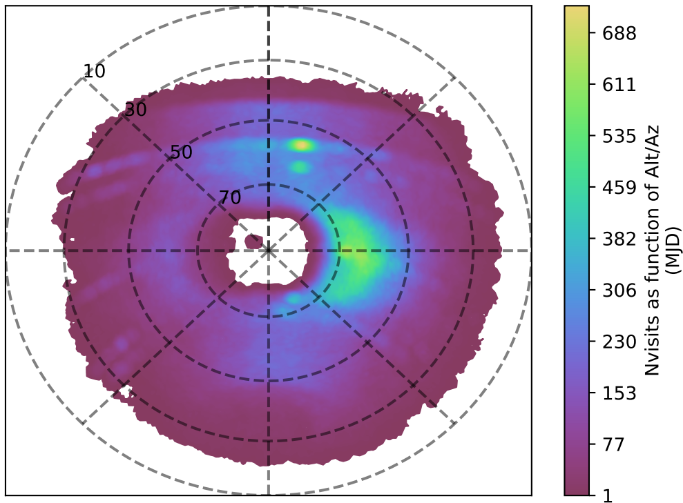
too_elab_r64_d2_gz_v3.4_10yrs u band: Nvisits as function of Alt/Az
