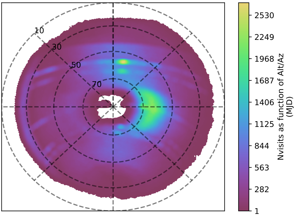
too_elab_r64_d2_gz_v3.4_10yrs r band: Nvisits as function of Alt/Az
