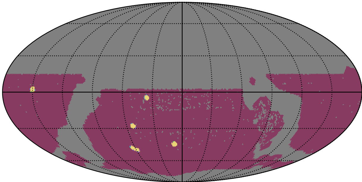
too_elab_r64_d2_gz_v3.4_10yrs WFD: NumberOfQuickRevisits
