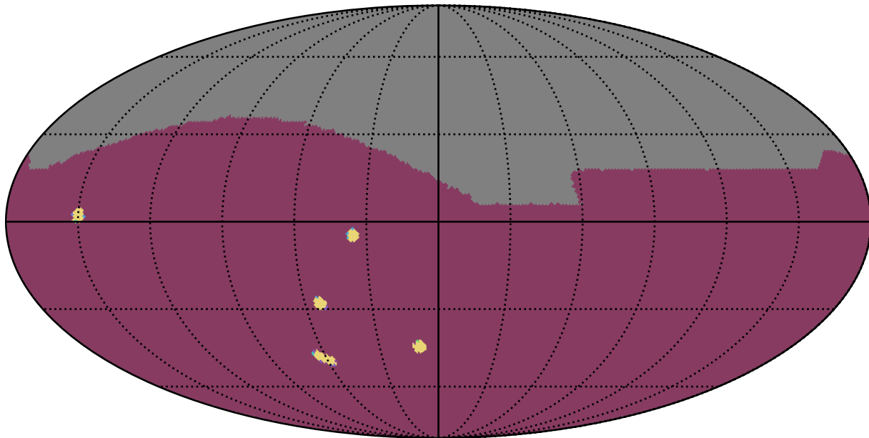
too_elab_r64_d2_gz_v3.4_10yrs All sky: NumberOfQuickRevisits
