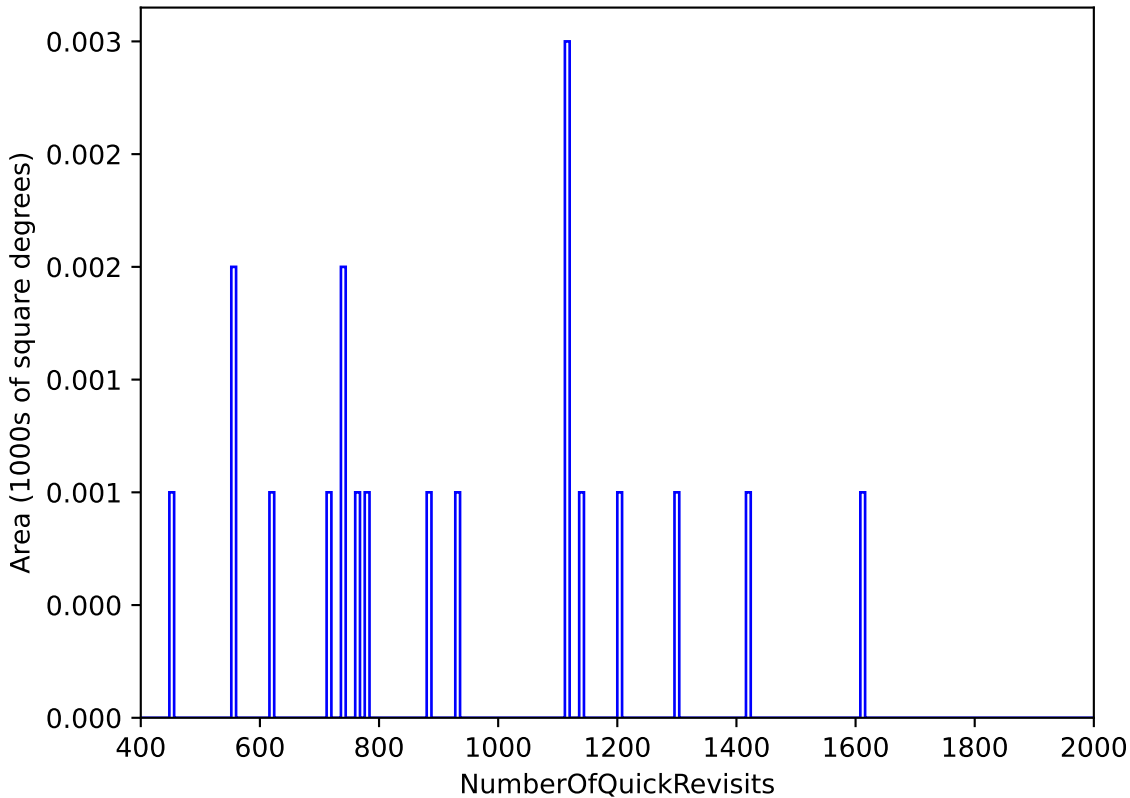
too_elab_r64_d2_gz_v3.4_10yrs All sky: NumberOfQuickRevisits
