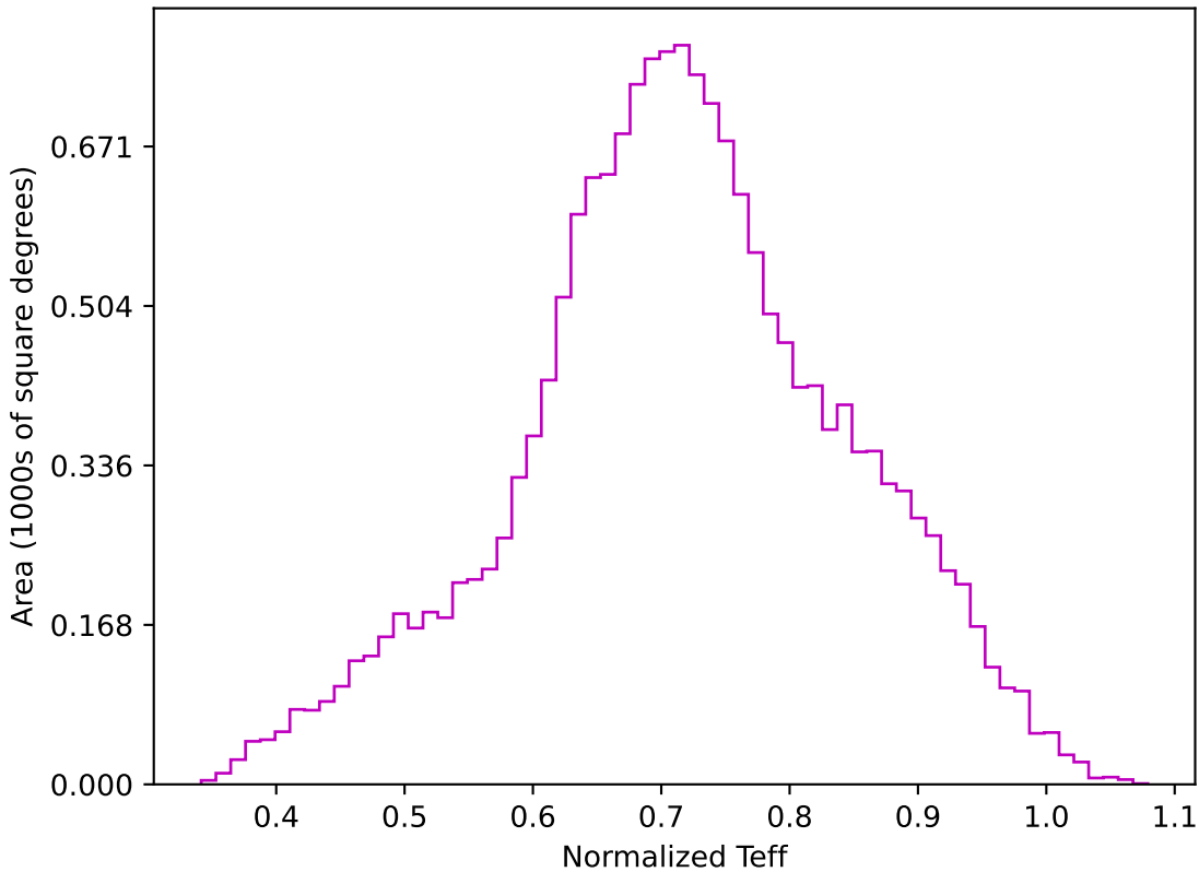
too_elab_r64_d2_gz_v3.4_10yrs WFD z band: Normalized Teff
