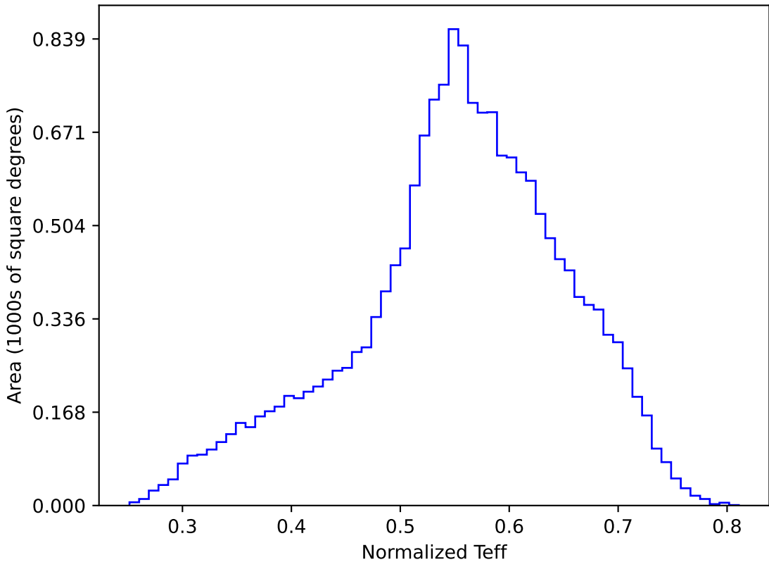
too_elab_r64_d2_gz_v3.4_10yrs WFD y band: Normalized Teff
