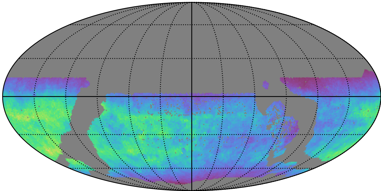
too_elab_r64_d2_gz_v3.4_10yrs WFD u band: Normalized Teff
