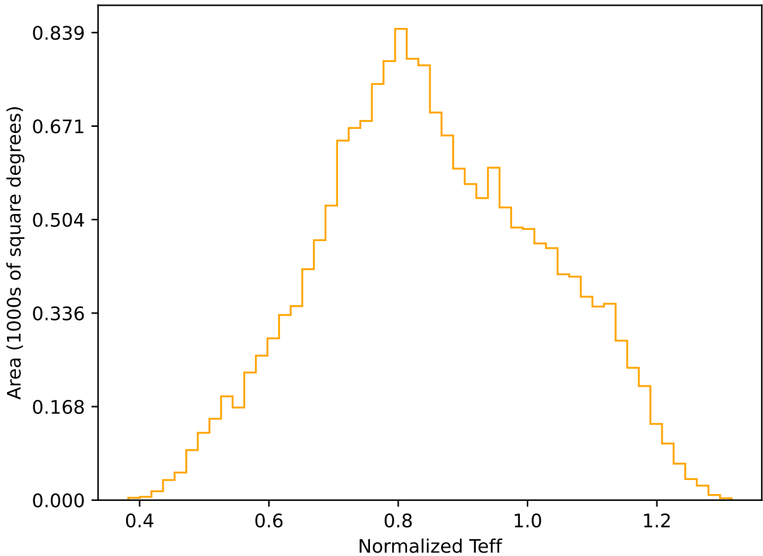
too_elab_r64_d2_gz_v3.4_10yrs WFD r band: Normalized Teff
