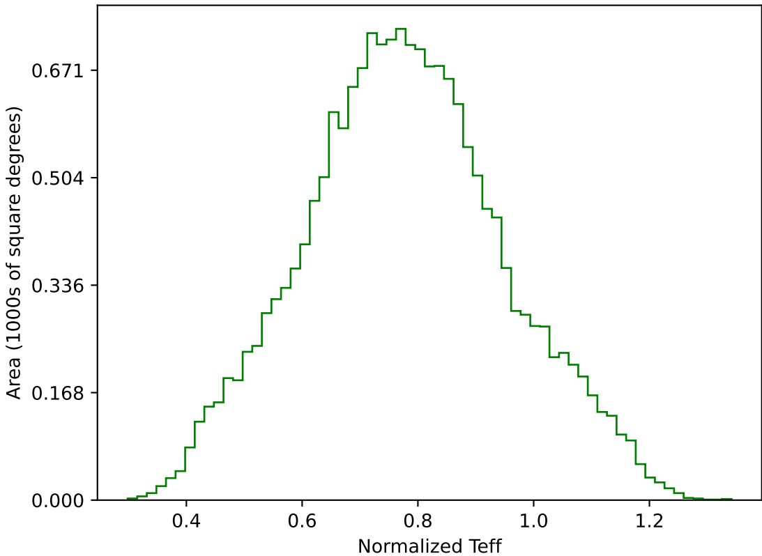
too_elab_r64_d2_gz_v3.4_10yrs WFD g band: Normalized Teff
