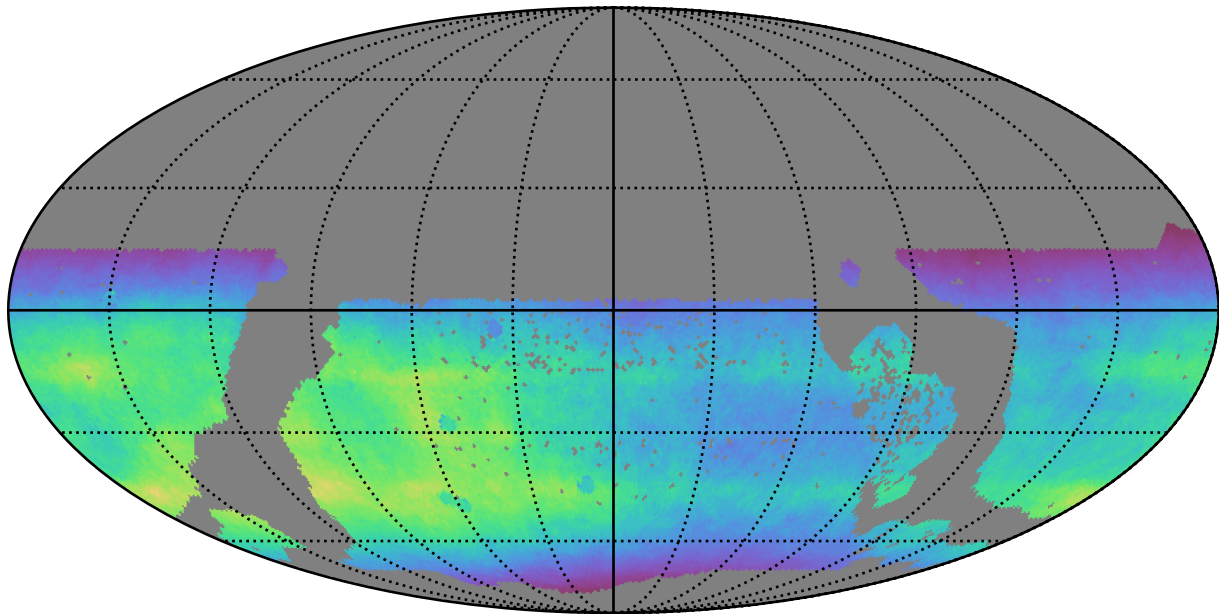
too_elab_r64_d2_gz_v3.4_10yrs WFD all bands: Normalized Teff
