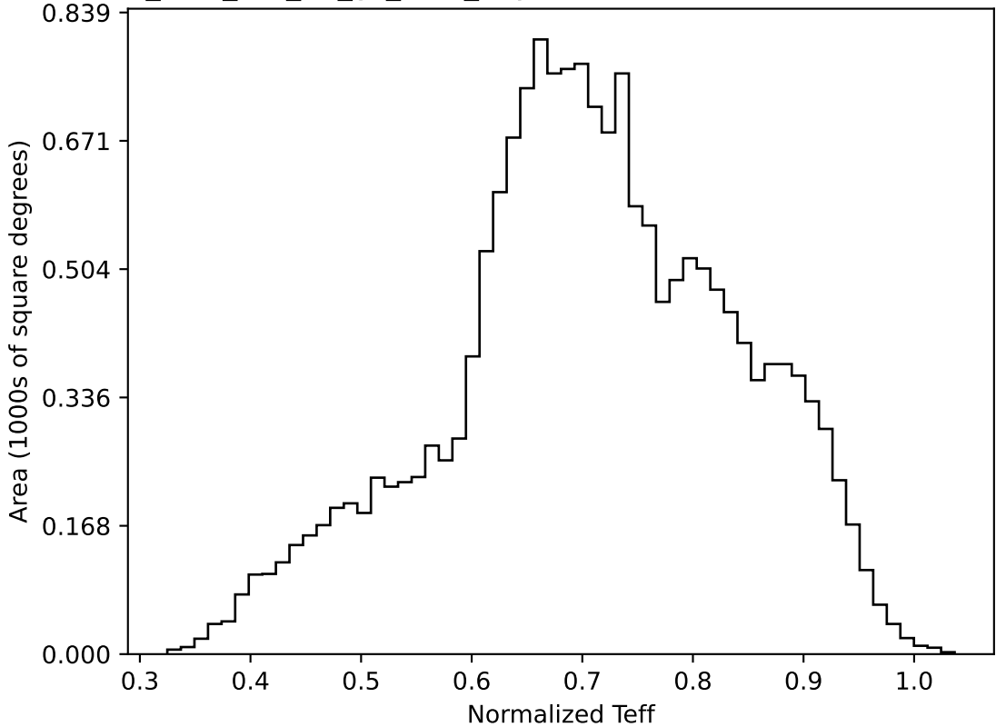
too_elab_r64_d2_gz_v3.4_10yrs WFD all bands: Normalized Teff
