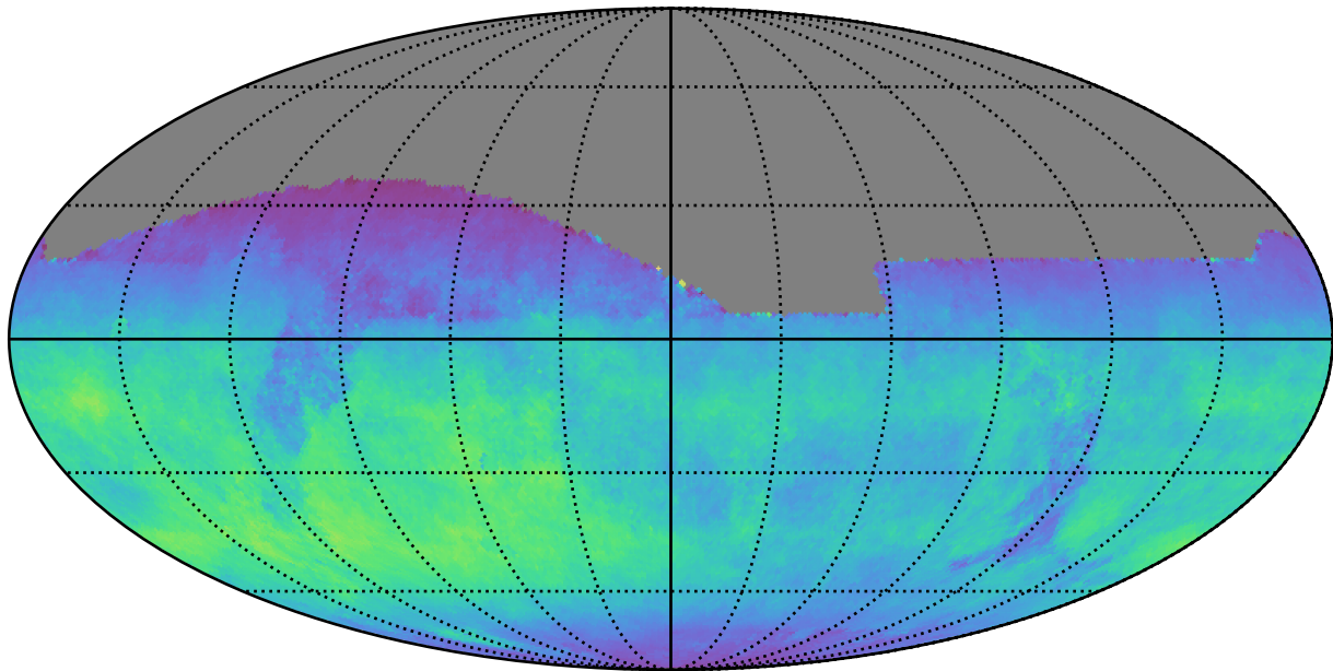
too_elab_r64_d2_gz_v3.4_10yrs All sky z band: Normalized Teff
