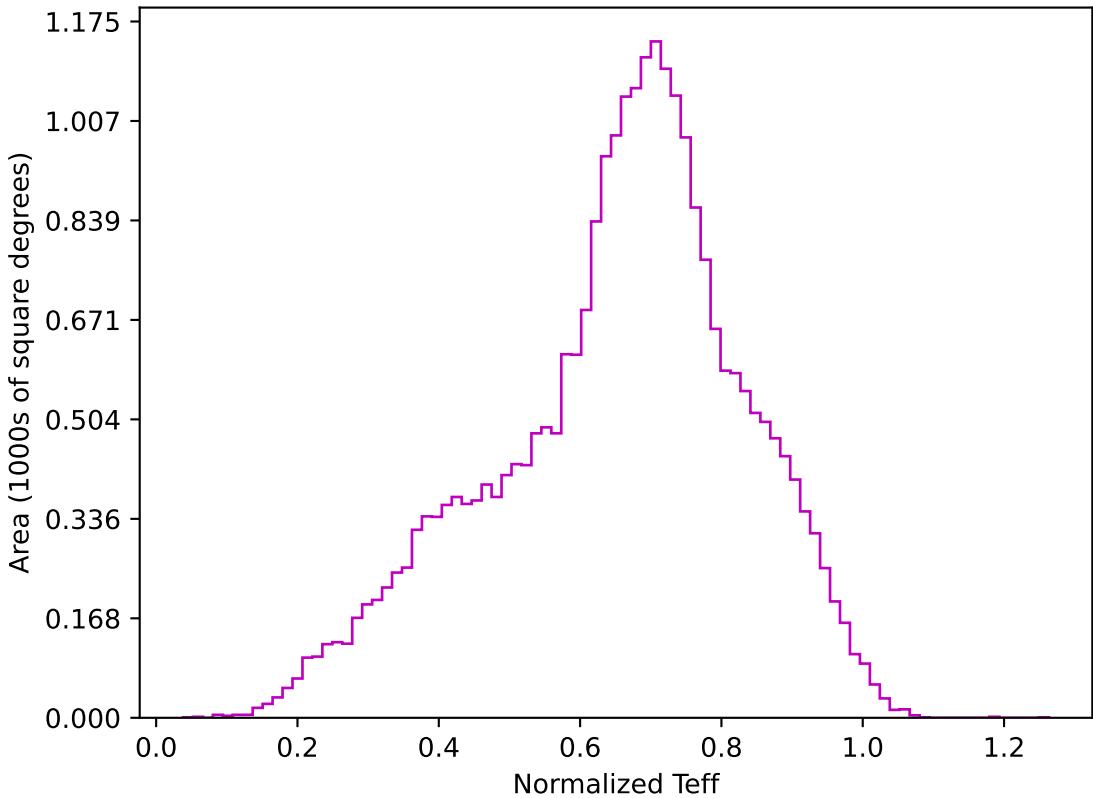
too_elab_r64_d2_gz_v3.4_10yrs All sky z band: Normalized Teff
