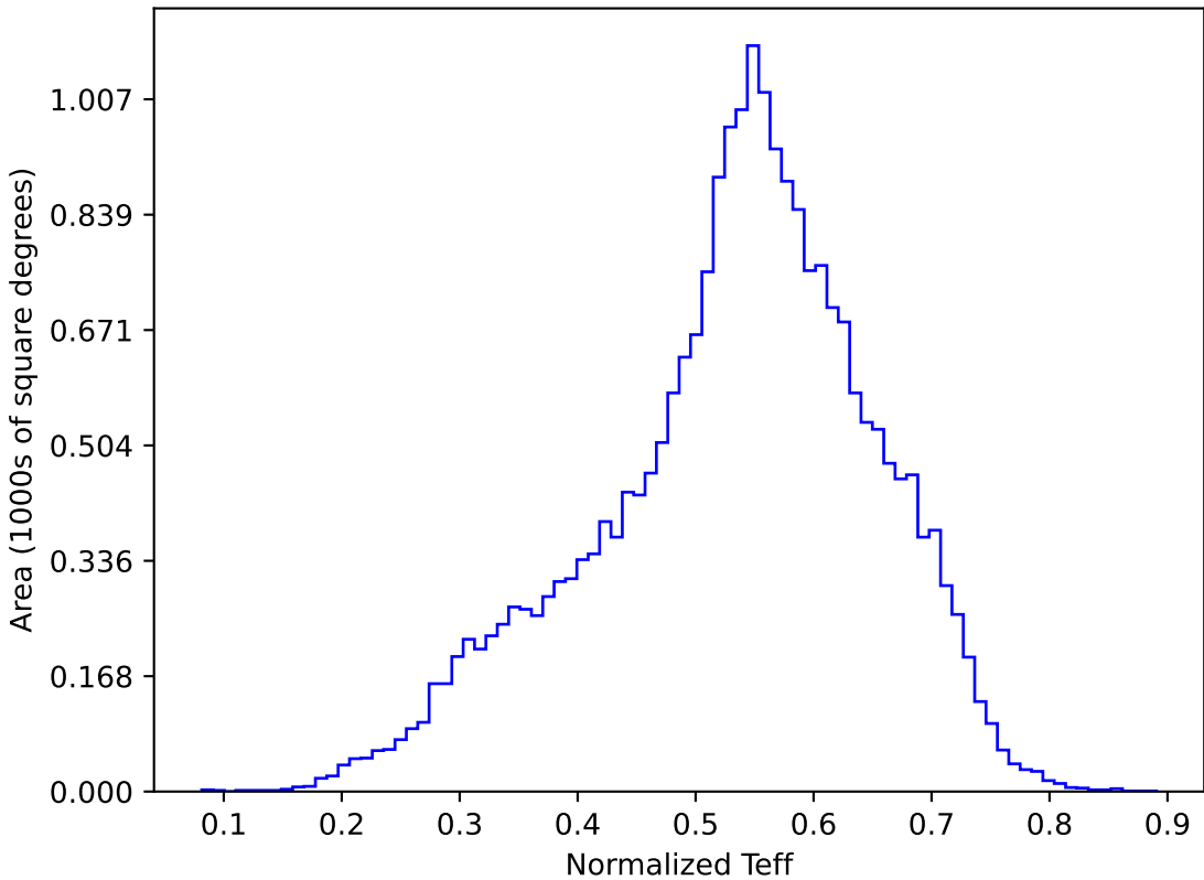
too_elab_r64_d2_gz_v3.4_10yrs All sky y band: Normalized Teff
