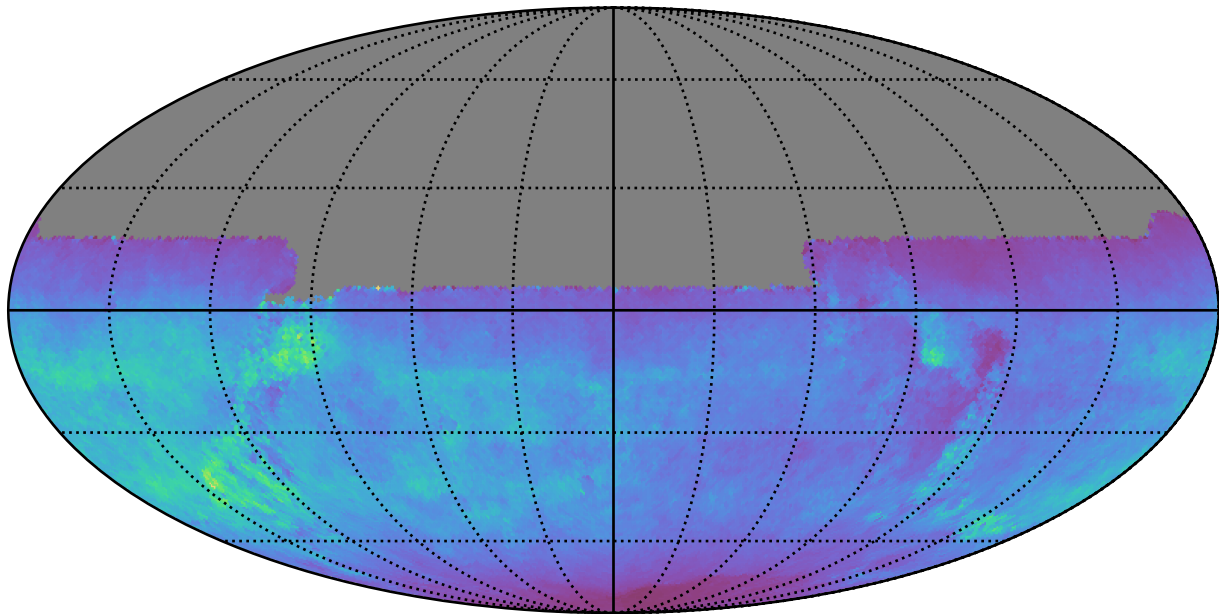
too_elab_r64_d2_gz_v3.4_10yrs All sky u band: Normalized Teff
