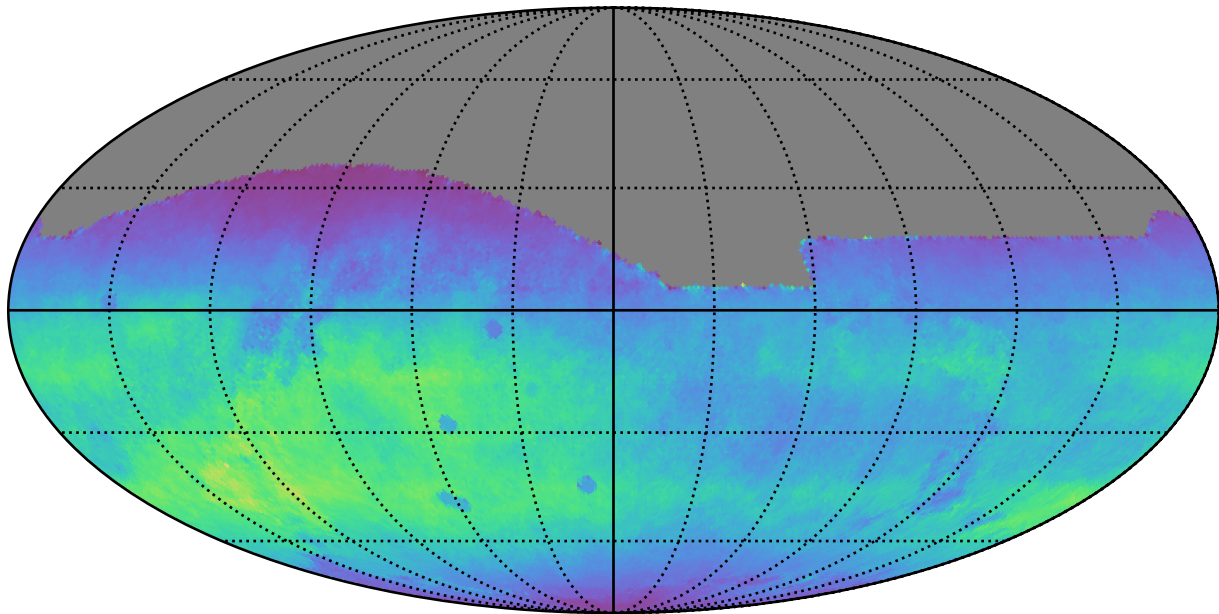
too_elab_r64_d2_gz_v3.4_10yrs All sky r band: Normalized Teff
