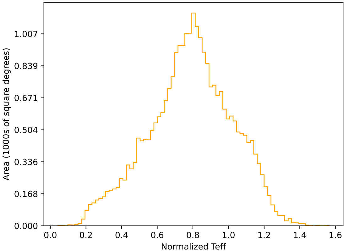
too_elab_r64_d2_gz_v3.4_10yrs All sky r band: Normalized Teff
