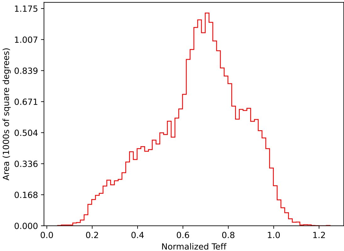
too_elab_r64_d2_gz_v3.4_10yrs All sky i band: Normalized Teff
