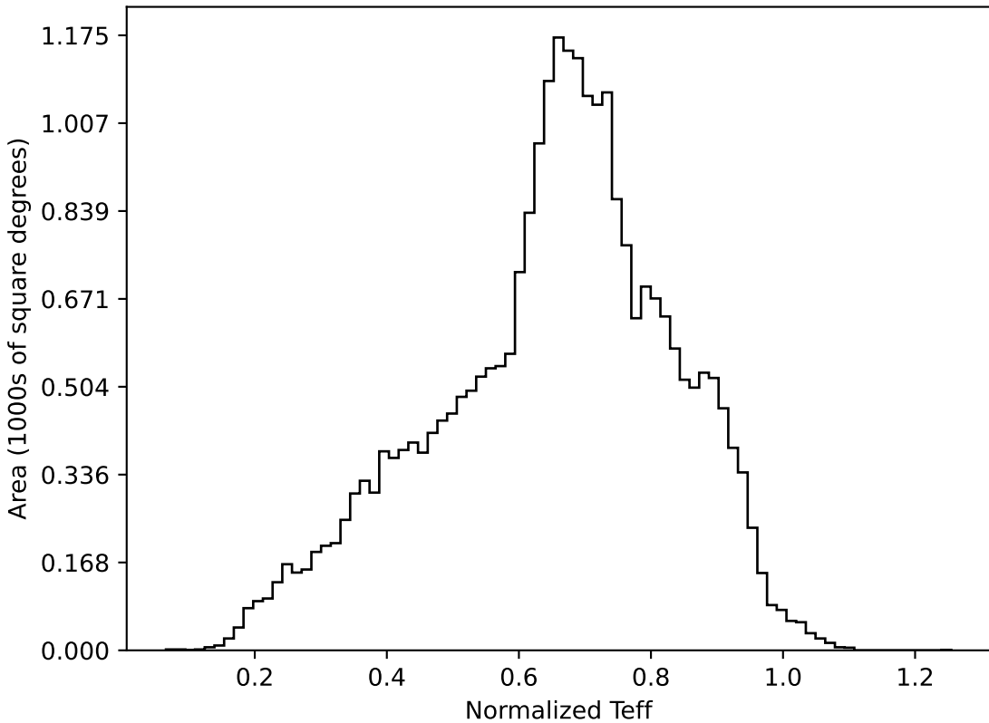
too_elab_r64_d2_gz_v3.4_10yrs All sky all bands: Normalized Teff
