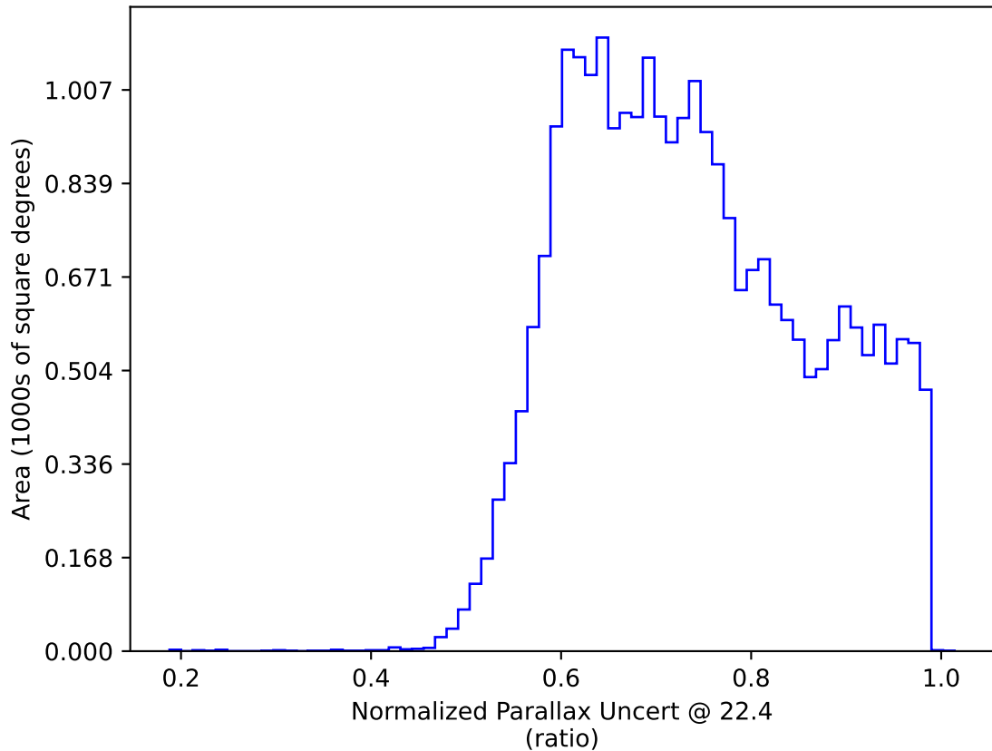
too_elab_r64_d2_gz_v3.4_10yrs All sky: Normalized Parallax Uncert @ 22.4
