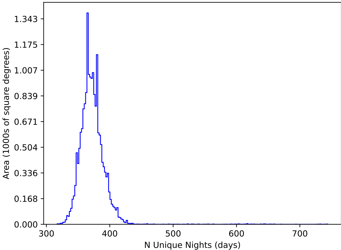
too_elab_r64_d2_gz_v3.4_10yrs WFD all bands: N Unique Nights
