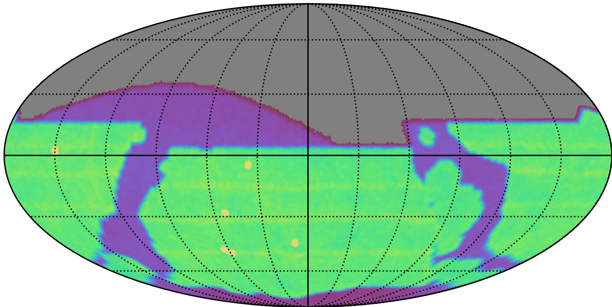
too_elab_r64_d2_gz_v3.4_10yrs All sky all bands: N Unique Nights
