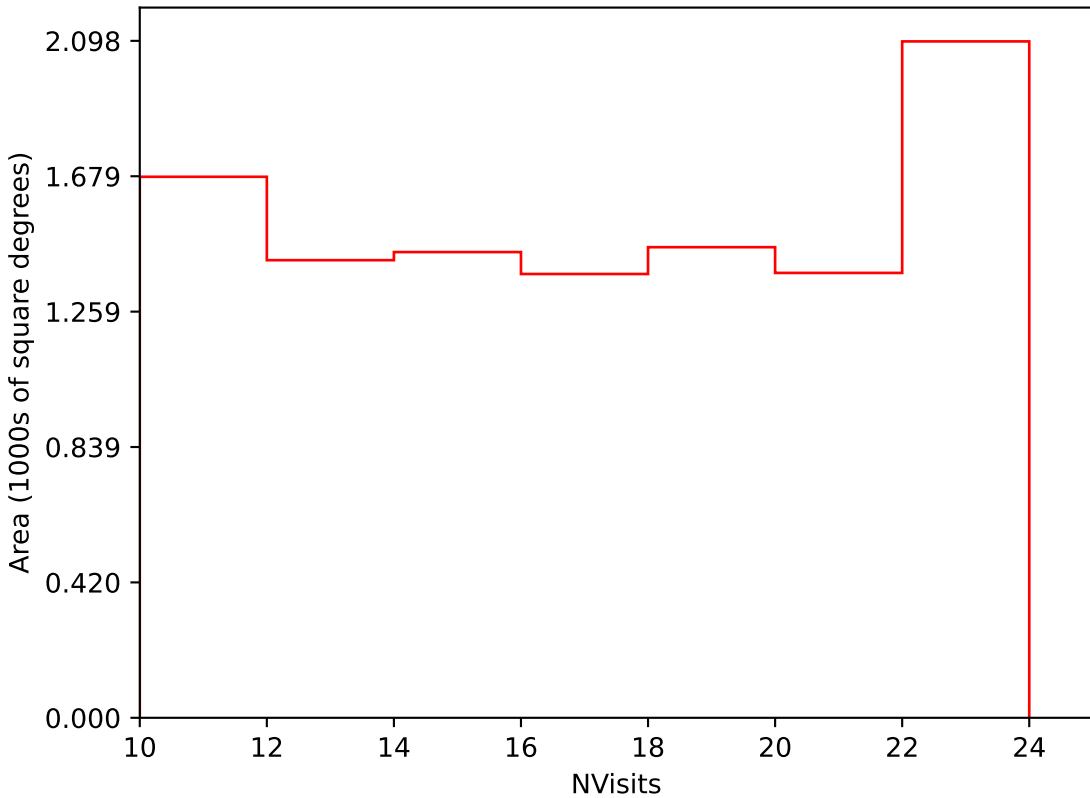
too_elab_r64_d2_gz_v3.4_10yrs Yr 3-4 i band: NVisits
