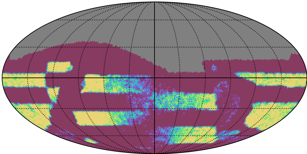
too_elab_r64_d2_gz_v3.4_10yrs Yr 3-4 all bands: NVisits
