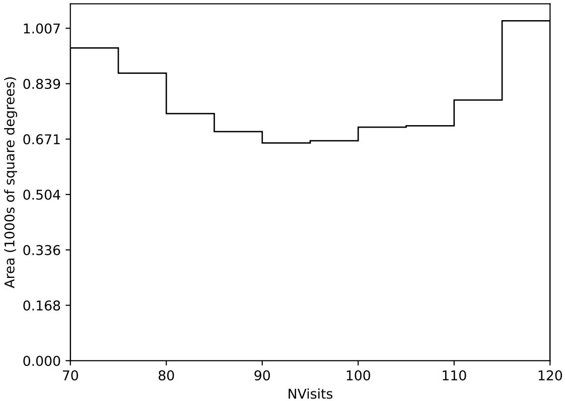
too_elab_r64_d2_gz_v3.4_10yrs Yr 3-4 all bands: NVisits
