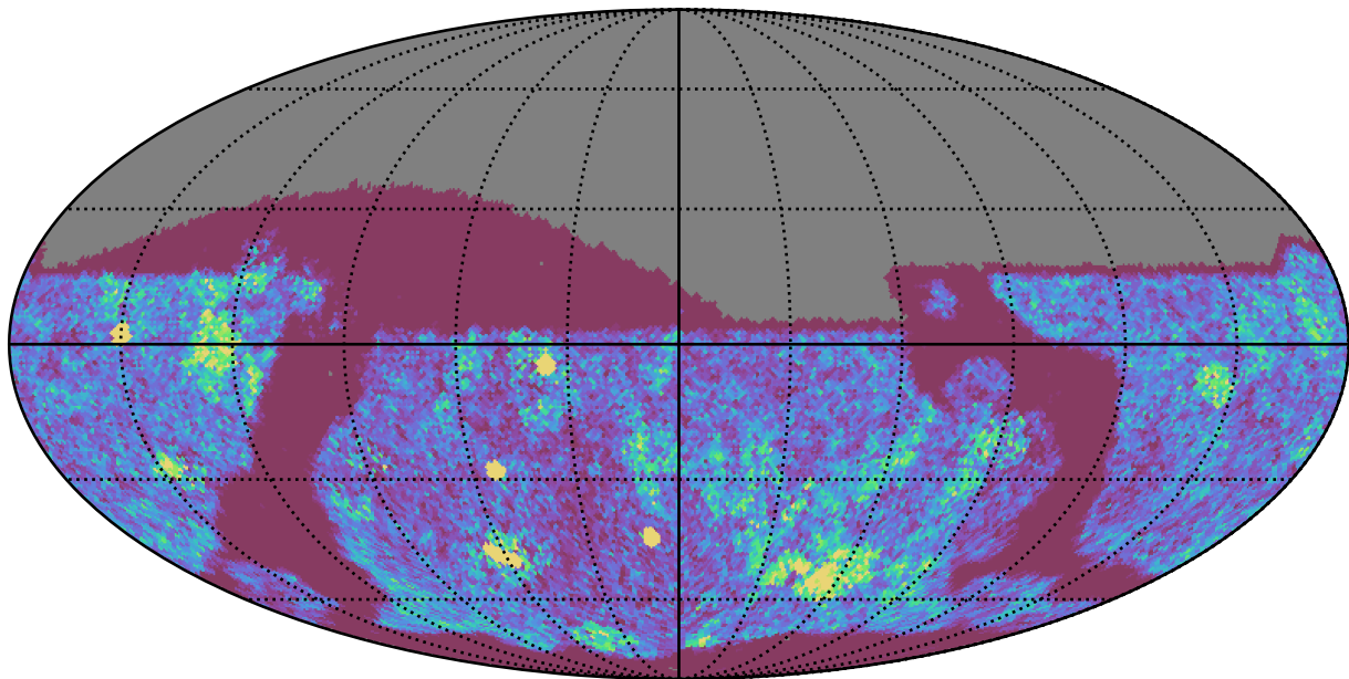
too_elab_r64_d2_gz_v3.4_10yrs Yr 1 z band: NVisits
