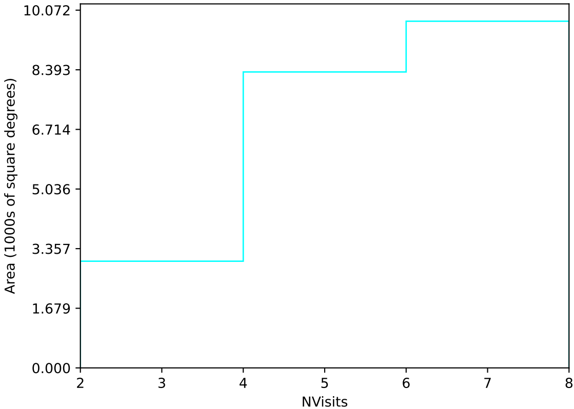
too_elab_r64_d2_gz_v3.4_10yrs Yr 1 u band: NVisits
