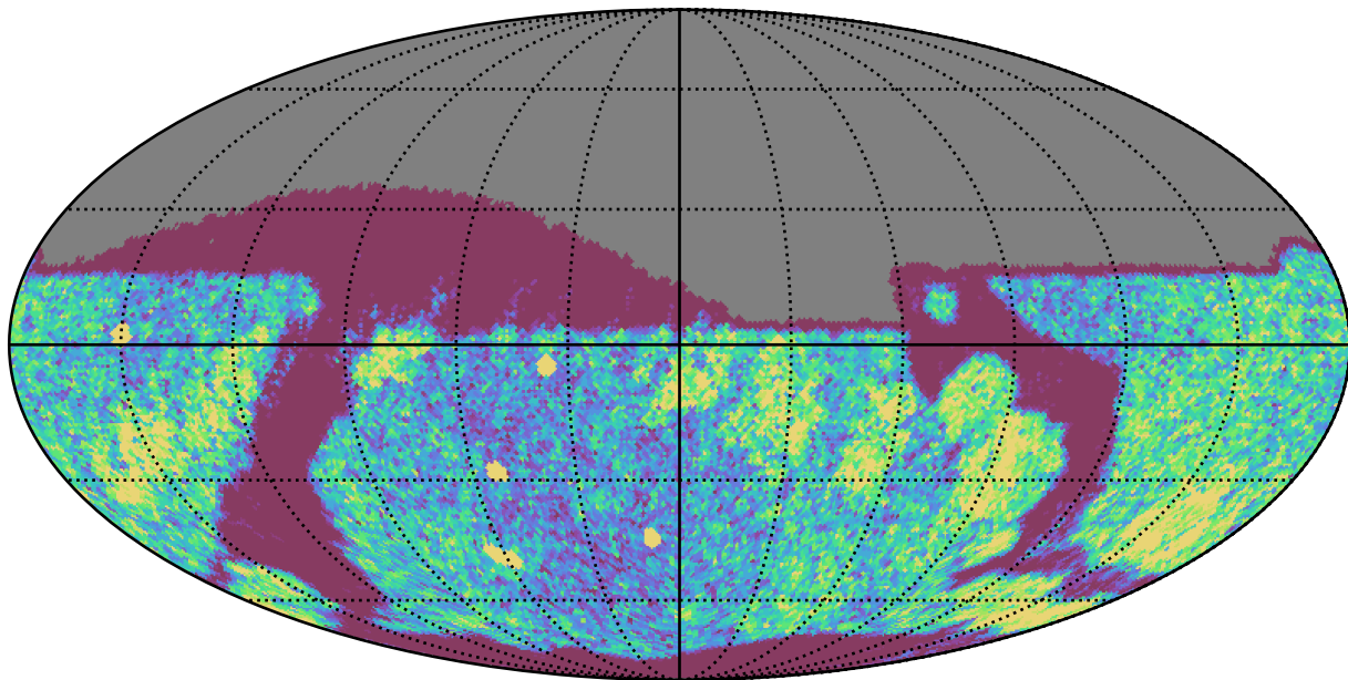
too_elab_r64_d2_gz_v3.4_10yrs Yr 1 r band: NVisits
