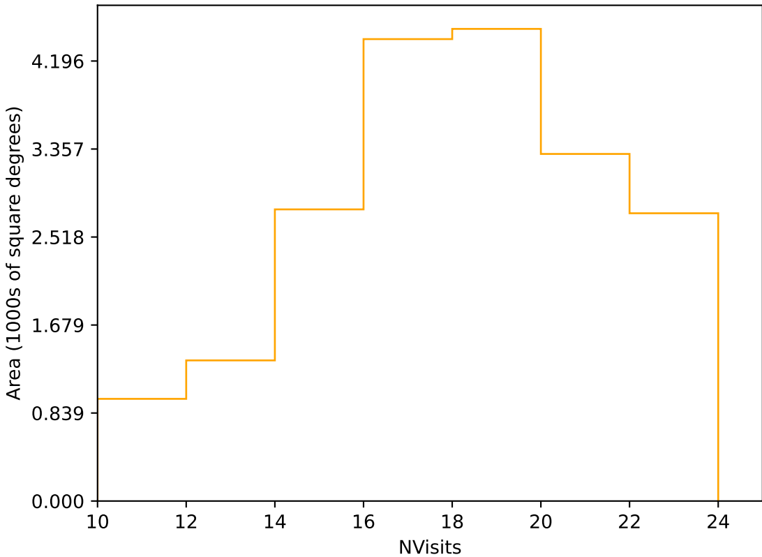
too_elab_r64_d2_gz_v3.4_10yrs Yr 1 r band: NVisits
