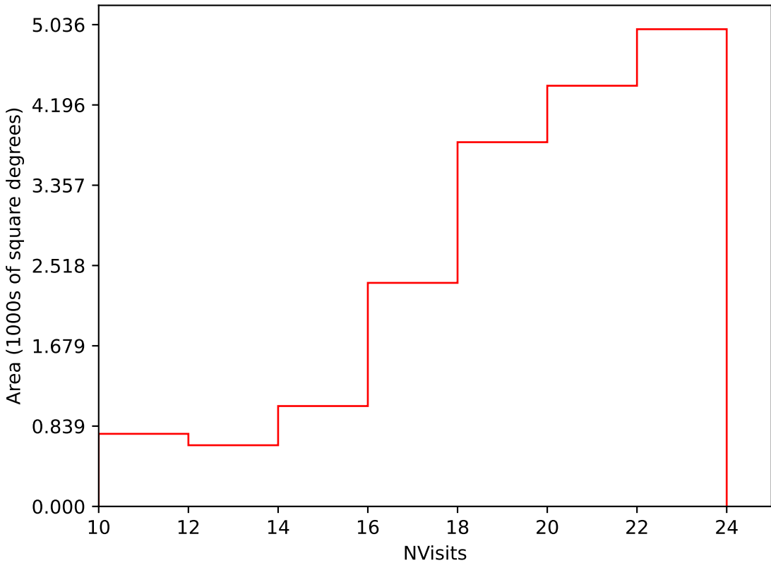
too_elab_r64_d2_gz_v3.4_10yrs Yr 1 i band: NVisits
