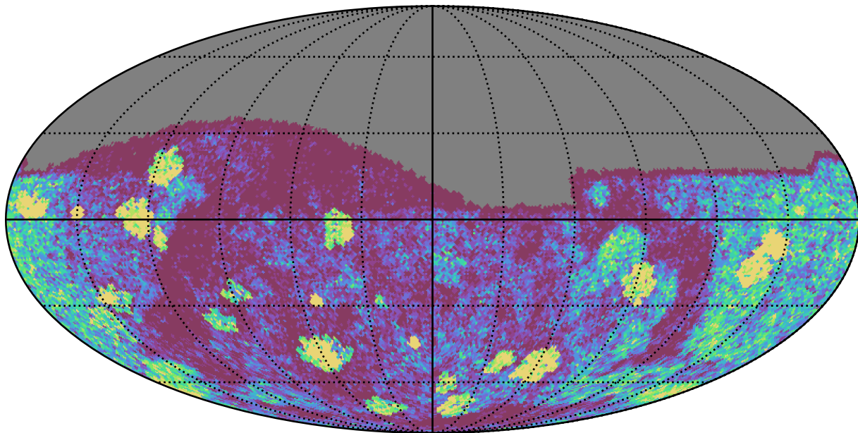
too_elab_r64_d2_gz_v3.4_10yrs Yr 1 g band: NVisits
